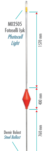
M02505 Fotoselli Işık Photocell Light Demir Balast Steel Ballast M03096 DAN BUOY
